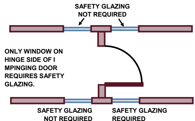
Hazardous Location for Glazing Adjacent to a Door
